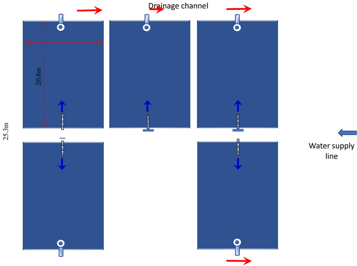
Figure 1: Proposed Pond Layout (Not to scale)
